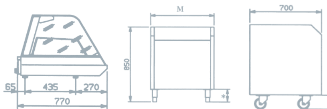
Dimensions-Side View
